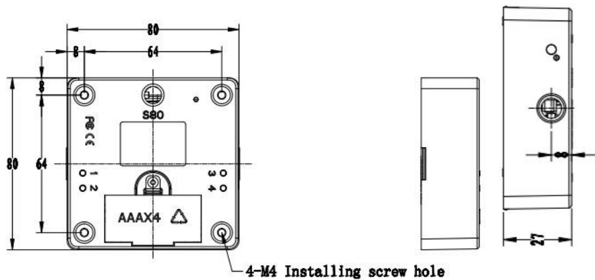
Lock body
